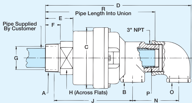
Type II Duoflow Fixed Pipe
