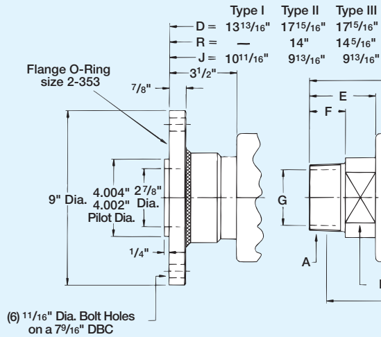
857-132 Flanged Rotor Detail
